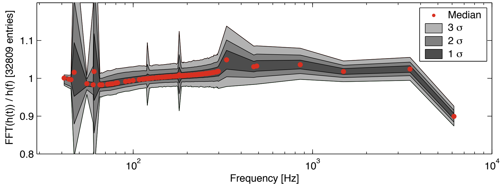
H1 !(GPS 835 to 840) comparison
