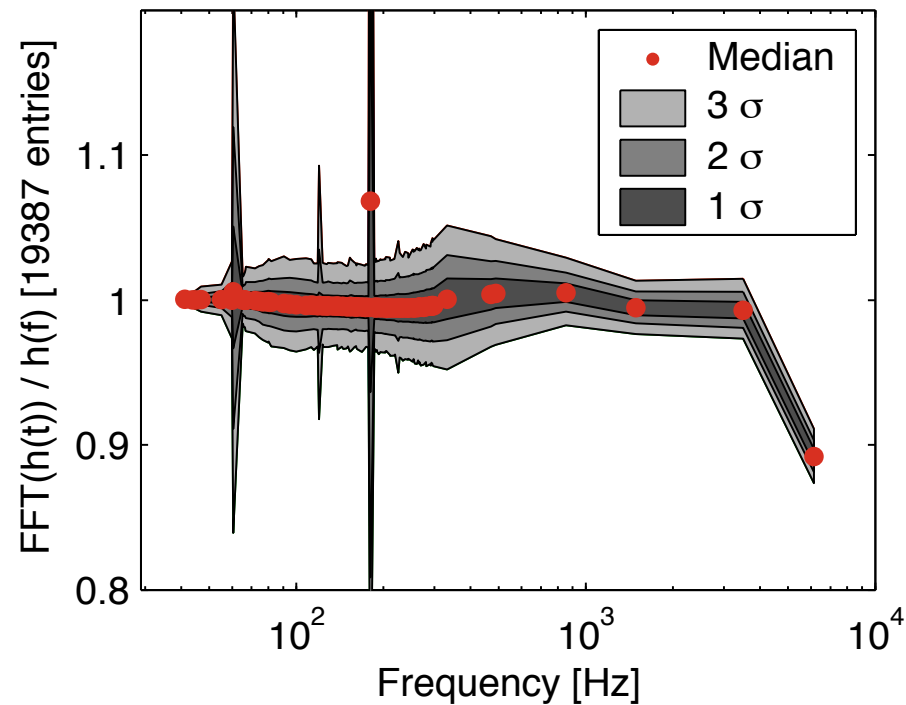
H2 Epoch 2 comparison
