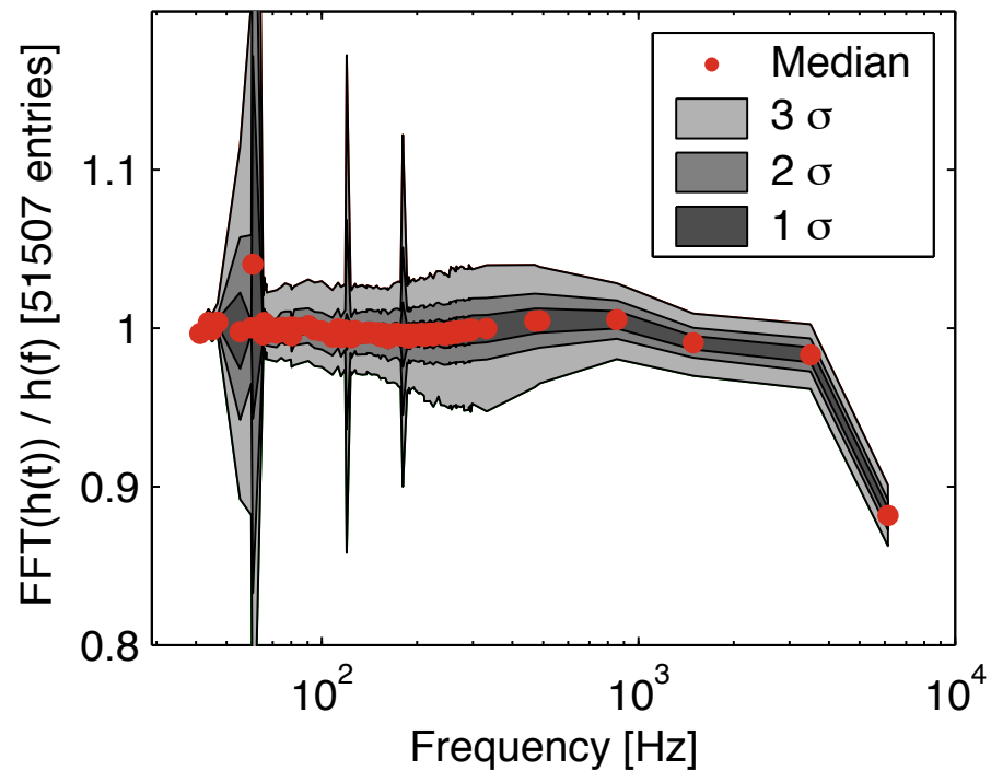
L1 Epoch 3 comparison
