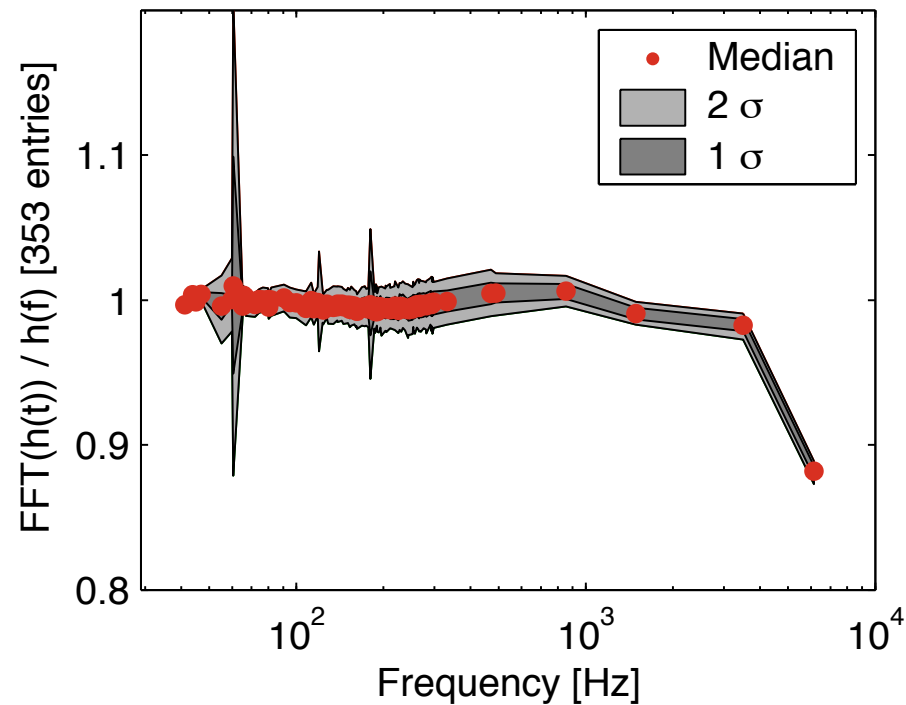
L1 Epoch 2 comparison
