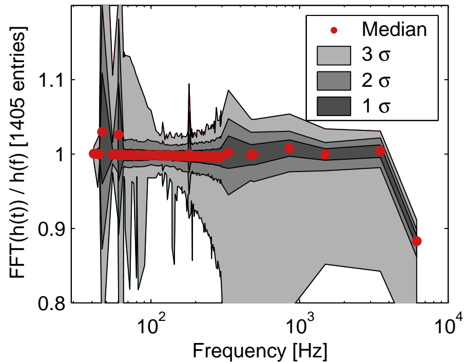
H1 Epoch 3 comparison
