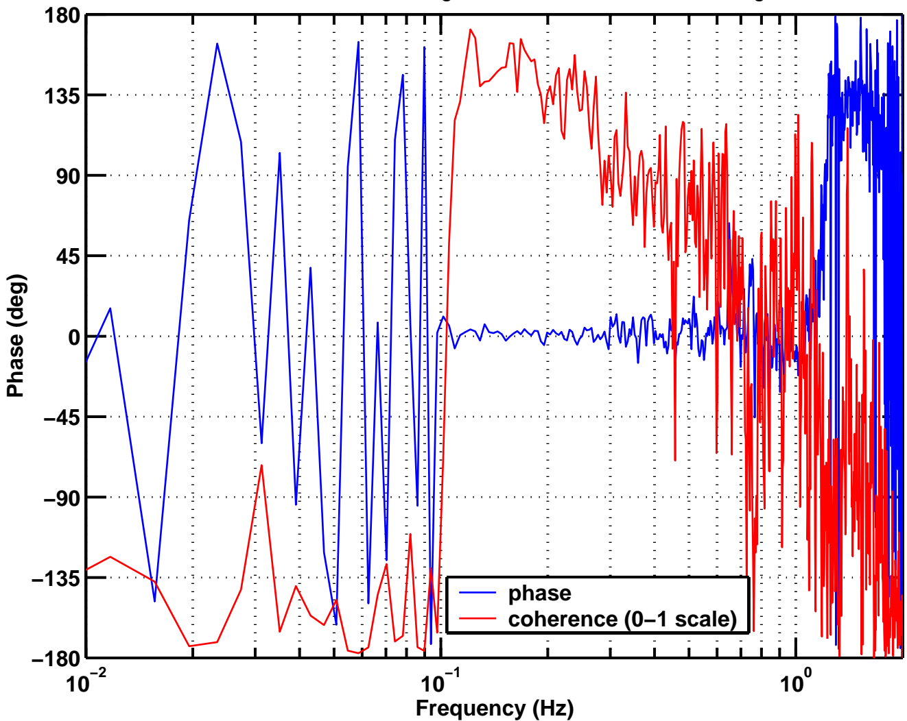
Phase & coh between Length control & seismometer diff signals
